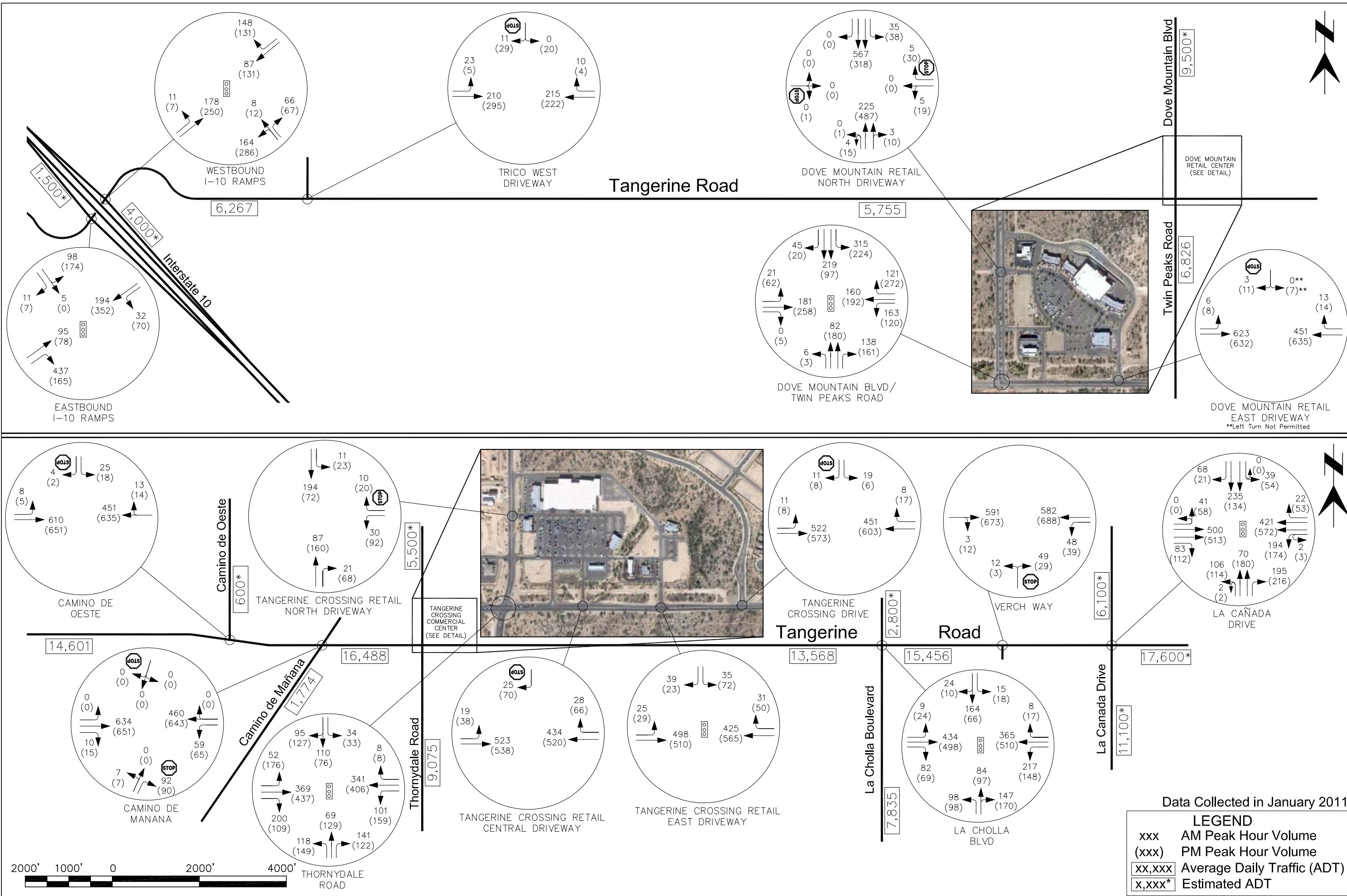
P S O M A S APRIL 2011 FIGURE X EXISTING TRAFFIC VOLUMES (2011) TANGERINE ROAD TRAFFIC ENGINEERING REPORT
