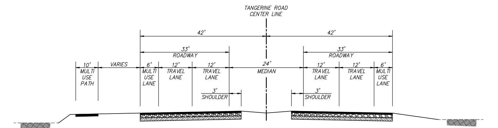
TANGERINE TYPICAL SECTION
