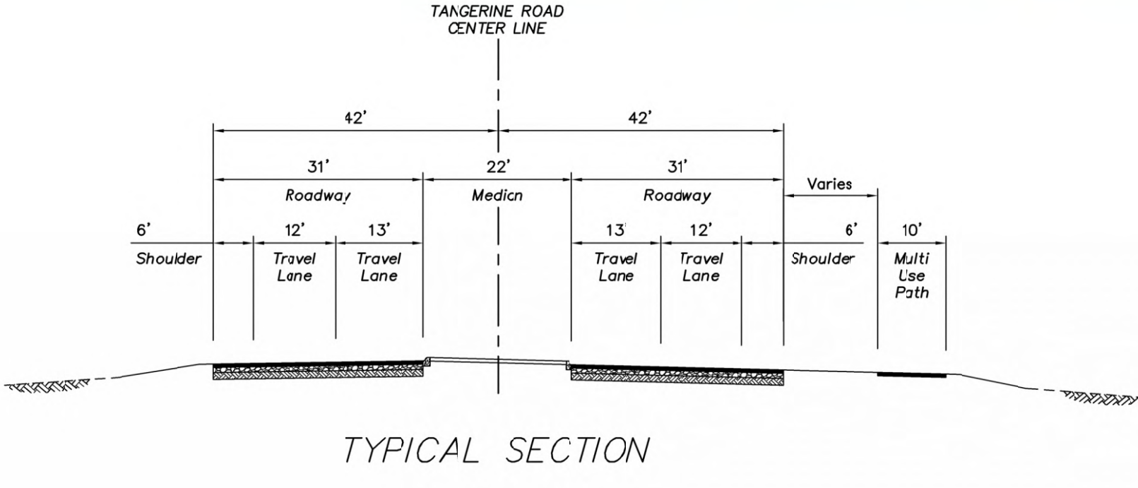
TYPICAL SECTION
